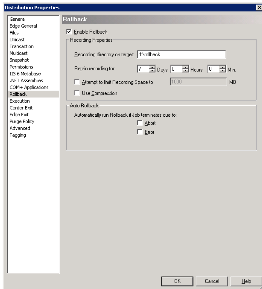
Figure 2: Rollback Definition
